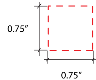
TOP IMPRINT
